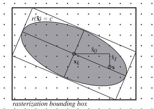
Fig. 12. Rasterizing the resampling filter.
