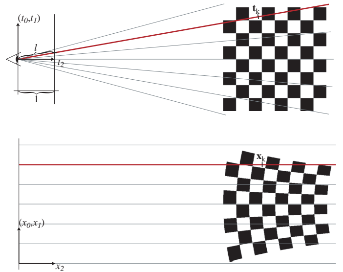
Fig. 8. Transforming the volume from camera to ray space. Top: camera space. Bottom: ray space.
