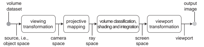
Fig. 4. The forward mapping volume rendering pipeline.
