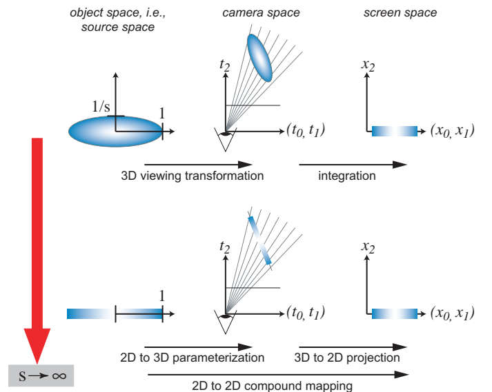
Fig. 10. Reducing a volume reconstruction kernel to a surface reconstruction kernel by flattening the kernel in one dimension. Top: rendering a volume kernel. Bottom: rendering a surface kernel.
