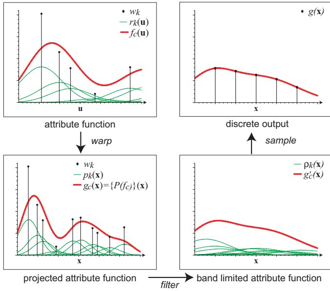
Fig. 3. Projection, filtering, and sampling of a 1D attribute function.
