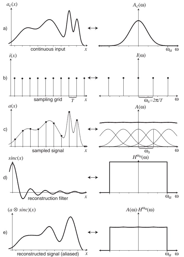
Fig. 2. Frequency analysis of aliasing.
