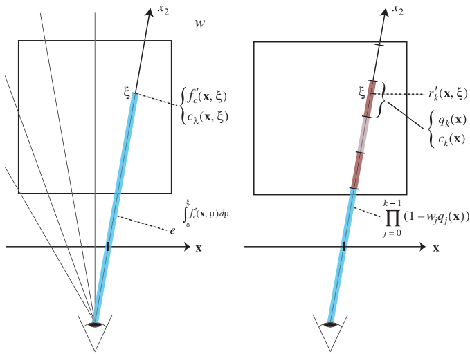
Fig. 5. Volume rendering. Left: Illustrating the volume rendering equation in 2D. Right: Approximations in typical splatting algorithms.
