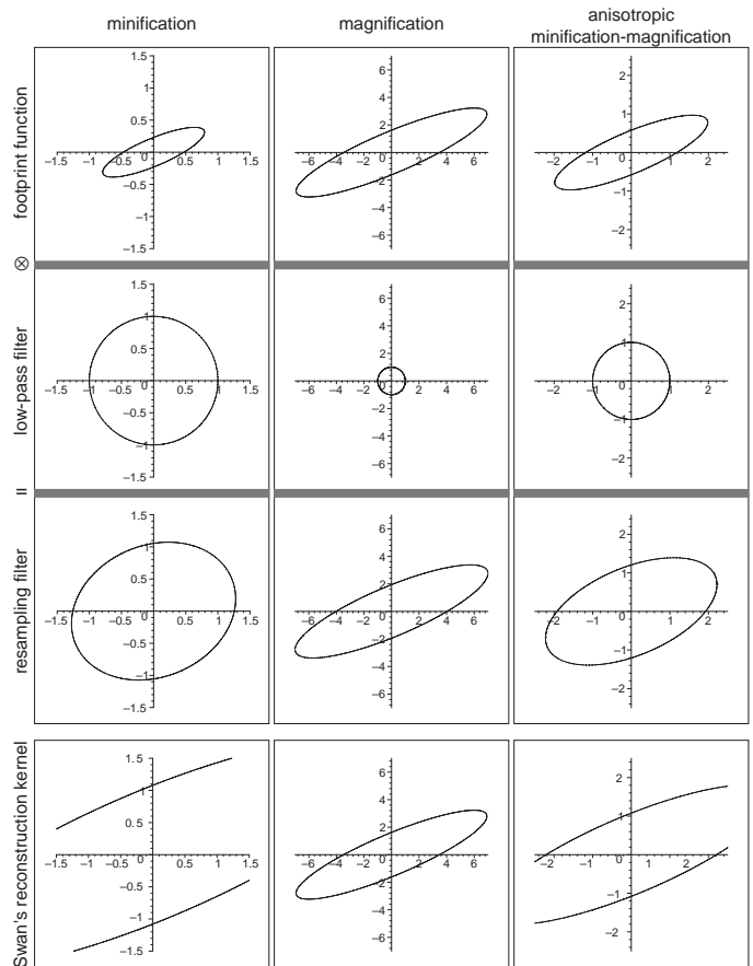
Fig. 13. Properties of the EWA resampling filter.
